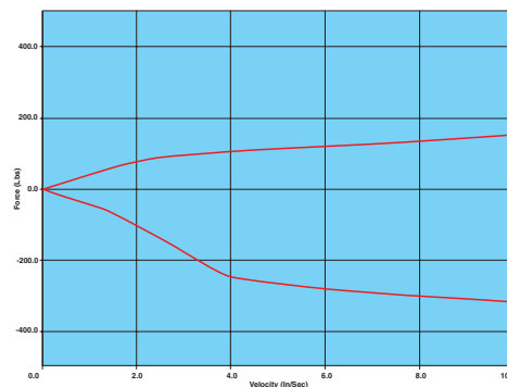
Shown here is a standard digressive valving using a low amount of bleed. Notice the large amount of force developed on both compression and rebound at slow piston speeds.
