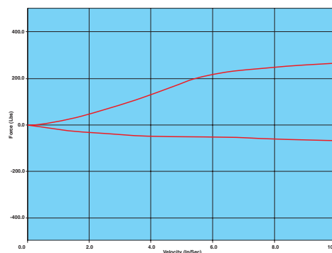
When the "COB" Digressive piston's check valve is installed on the rebound side, there is less bleed and therefore more force created on the compression side.
