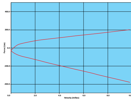
This graph depicts the BILSTEIN linear piston combined with 37.4mm cover plates. The result is valving with more "low-speed" control.
